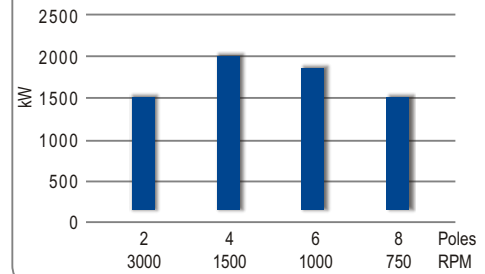
NG-Series Output Chart, Upto 13.2KV, 50Hz
