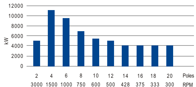
UD Series Output Chart, Upto 13.2KV, 50Hz
