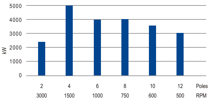
TV Series Output Chart, Upto 13.2KV, 50Hz
