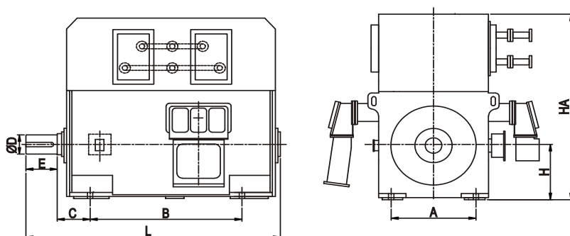
General Arrangement Drawing
