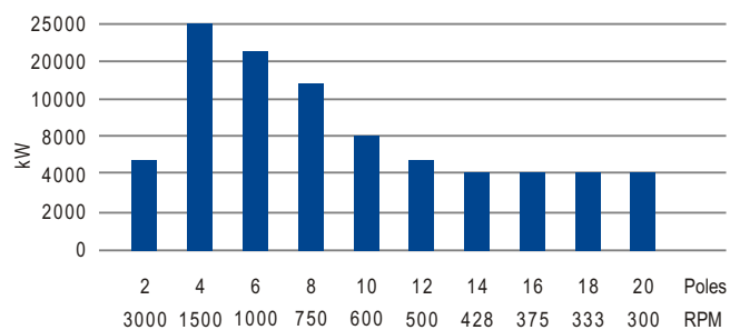
Output Chart, Upto 13.2KV, 50/60Hz
