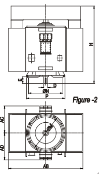
General Arrangement Drawing
