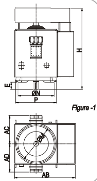
General Arrangement Drawing
