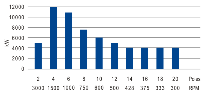
UW Series Output Chart, Upto 13.2KV, 50Hz
